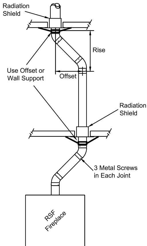
Figure 9 Offset Chimney Installation Example
