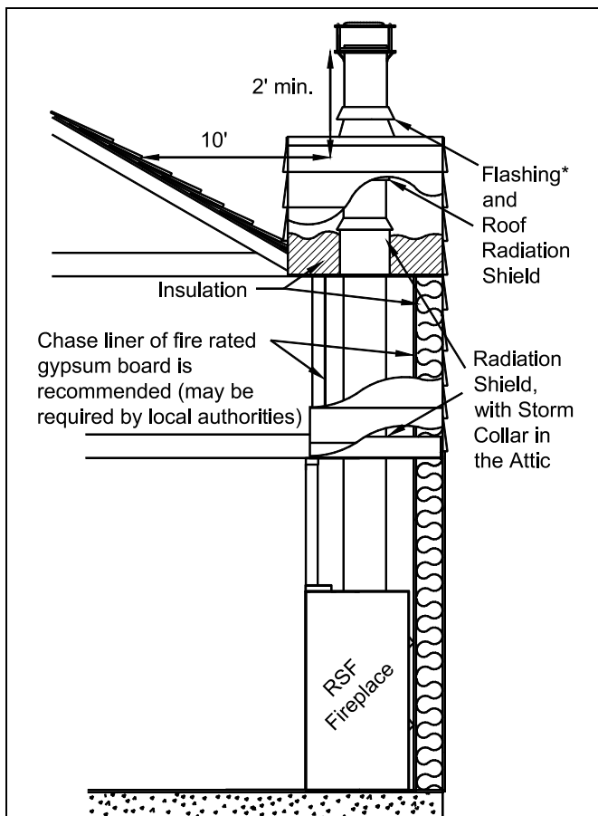
Figure 11 Chimney Installed with a Chase Enclosure Example
