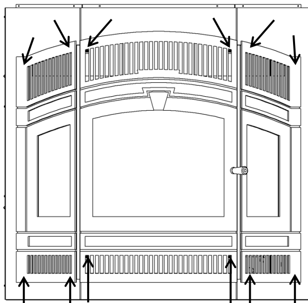
Figure 2 Top Louver, Bottom Louver and Side Decorative Facings Attachment
