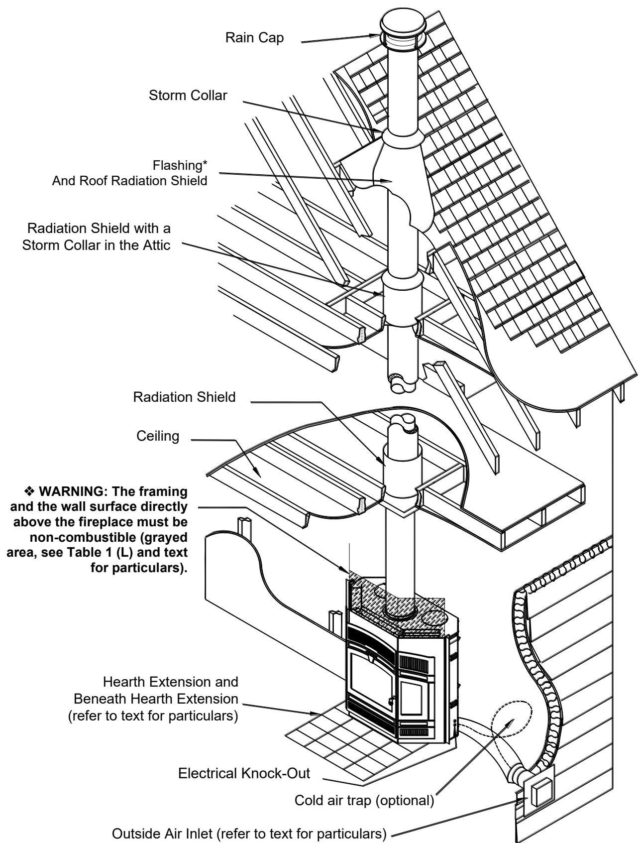
Figure 4 General Installation
