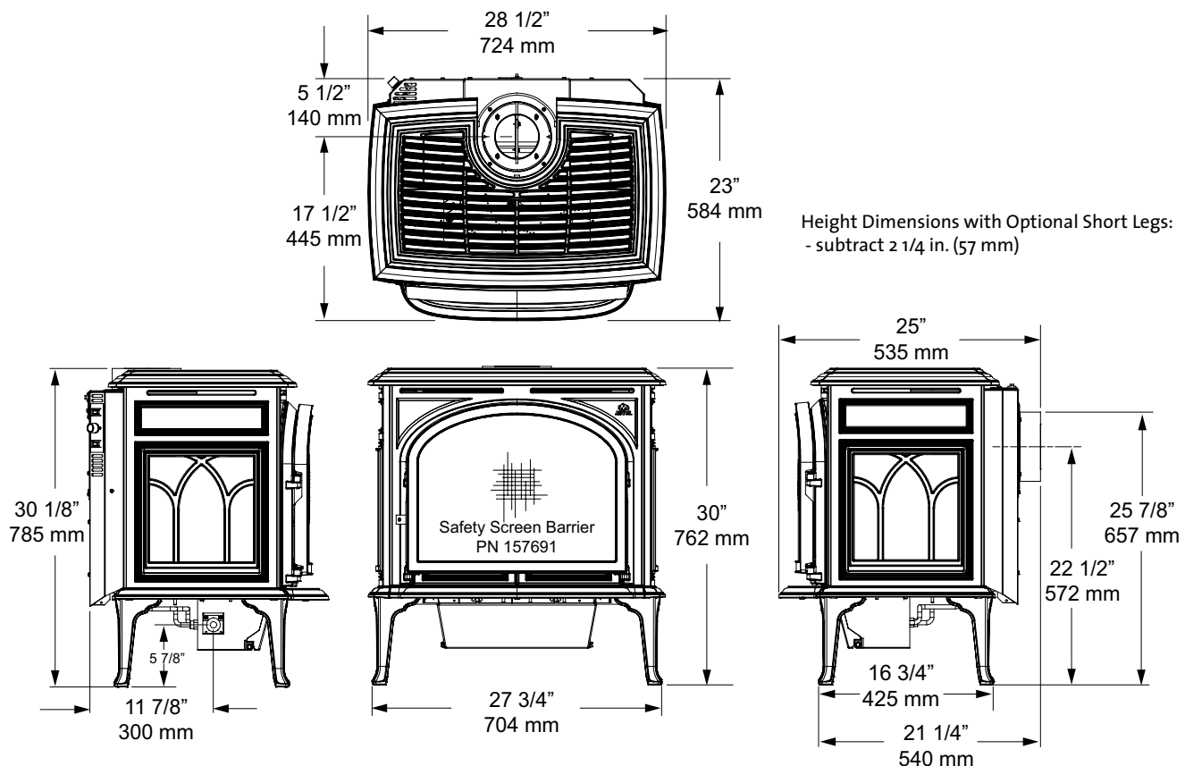
Figure 1. Dimensioned views, GF 500 DV MV
