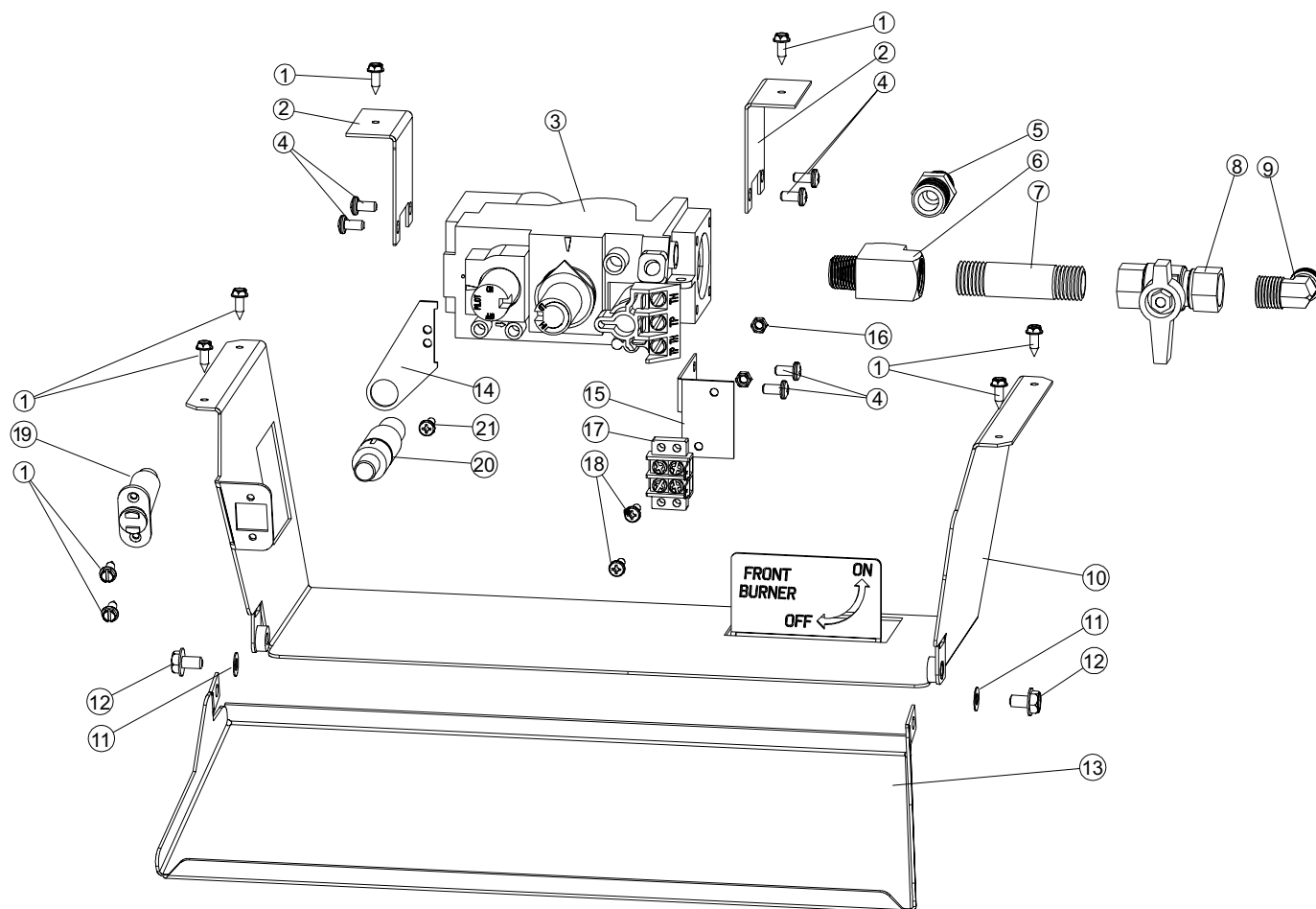
Figure 57. GF 500 DV MV Millivolt Valve components.
