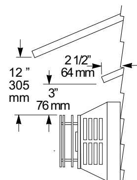
Figure 25. Termination Clearance to overhangs.
