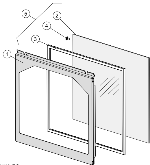
Figure 59. GF 500 DVMV Glass Assembly
