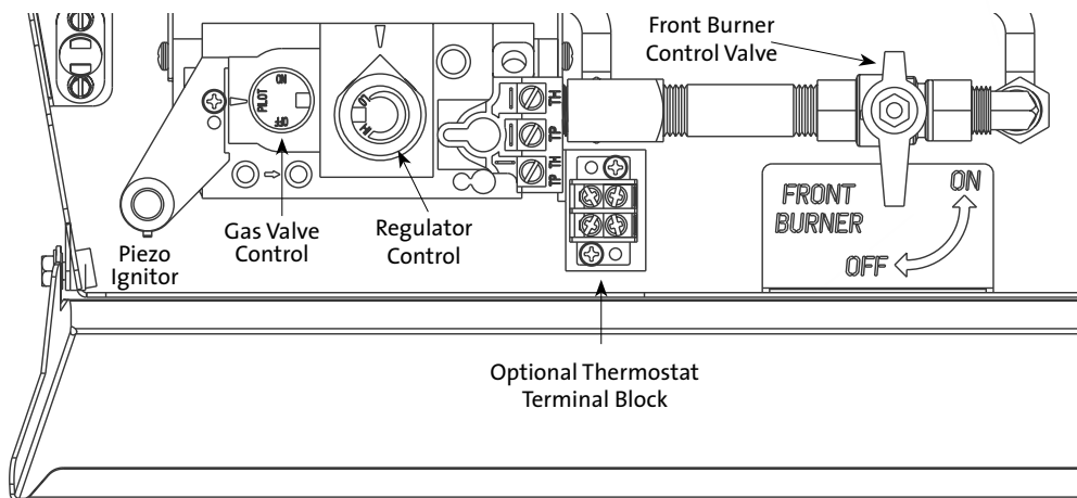
Figure 53. GF 500 DV MV Controls Compartment.
