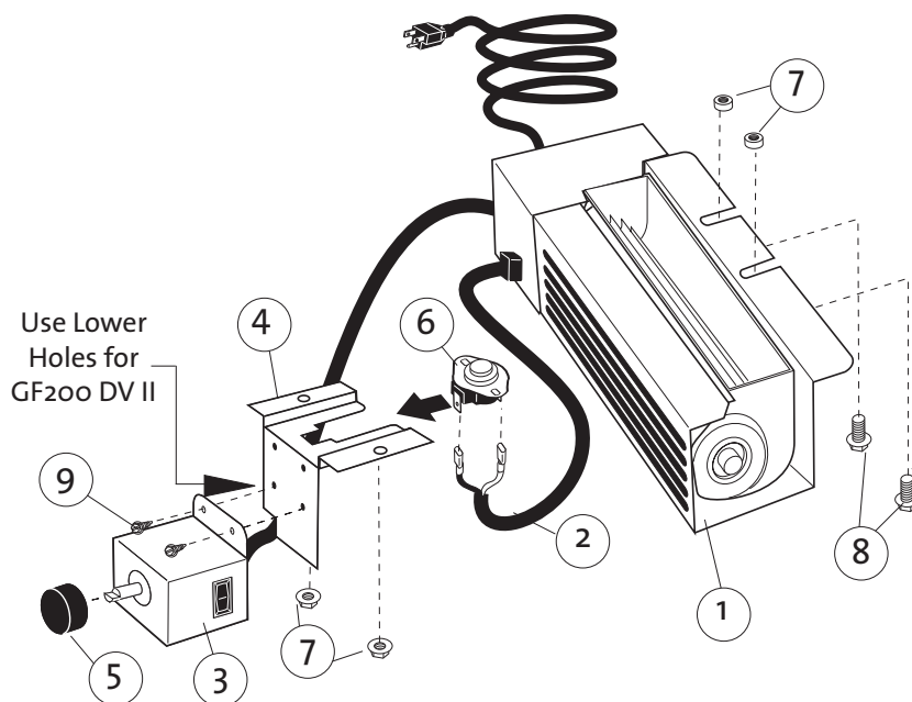
Figure 51. Blower Kit Components
