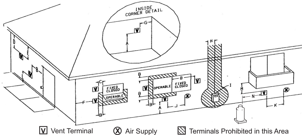
Figure 23. Vent Terminal Clearances - ANSI Z21.88-2009, CSA 2.33-2009, and National Fuel Gas Code.
