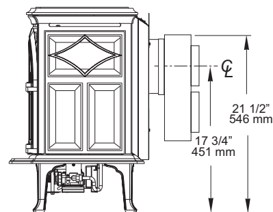
Figure 17. Simpson Dura-Vent #923GCL Co-linear Adaptor.
