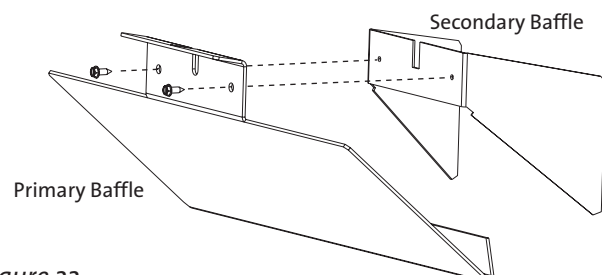
Figure 22. Use 1/4" (6 mm) socket driver to remove Primary Baffle from Secondary Baffle.
