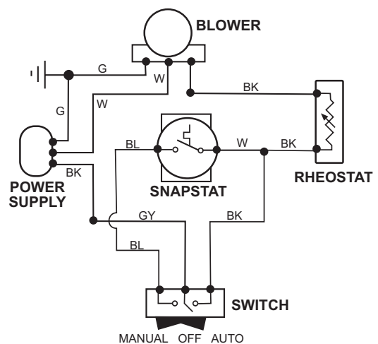
Figure 53. GF 200 DV IPI Blower Wiring Diagram.
