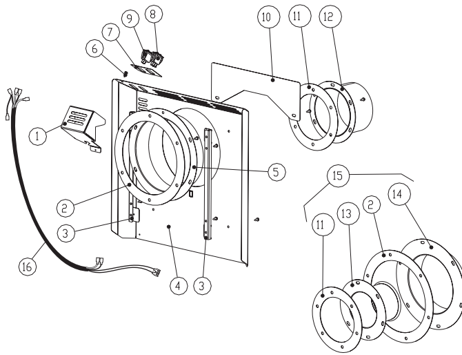
Figure 58. GF 200 DV IPI Rear Components
