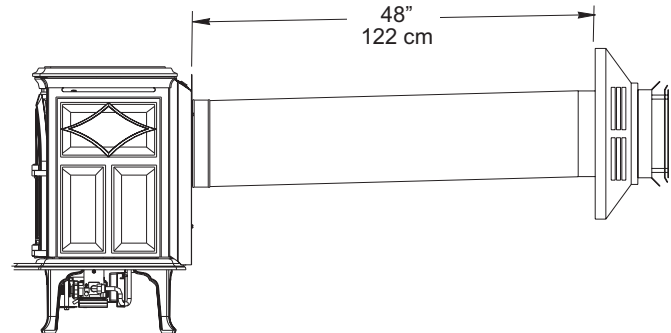
Figure 20. 5/8 Vent - Maximum horizontal vent - no vertical run. 1/4 inch (6mm) rise per foot is required.
