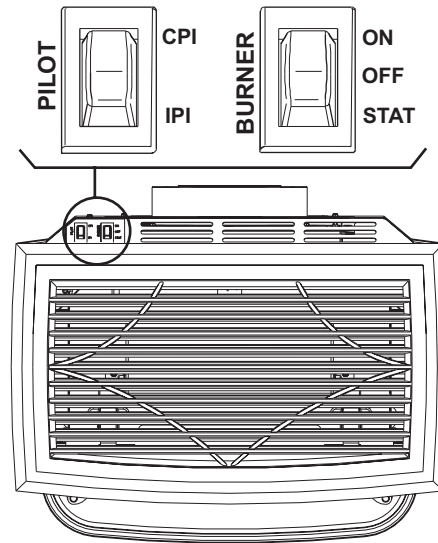
Figure 48. Burner controls location, viewed from above stove.
