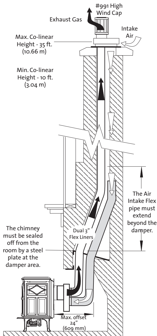
Figure 16. Co-linear Adaptor installed through a masonry chimney. Simpson Dura-Vent components shown.
