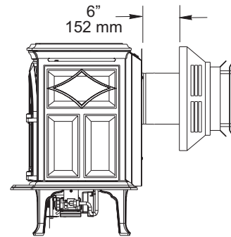
Figure 19. Minimum vent for horizontal termination.
