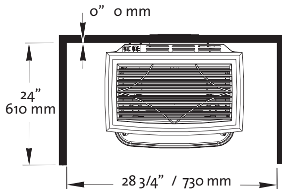
Figure 4. Minimum Alcove Clearances.
