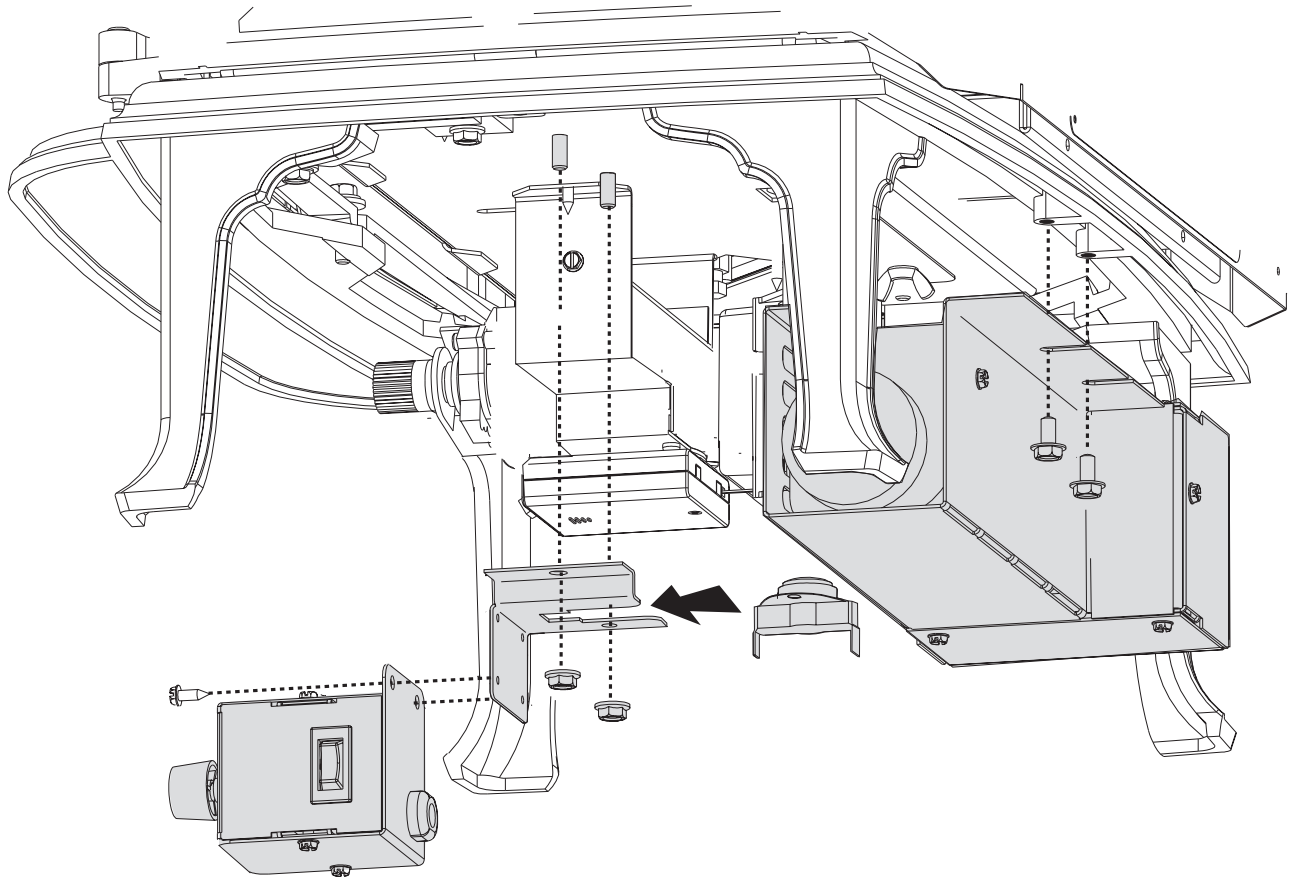
Figure 52. 155631 Blower Kit Components used for GF 200 DV IPI Lillehammer.
