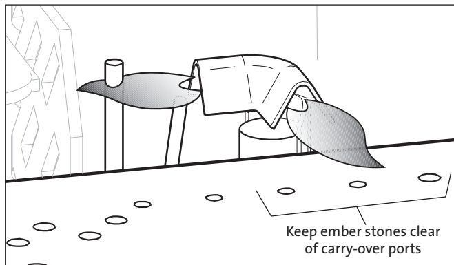
Figure 43. Proper pilot flame appearance relative to burner carry-over porting.
