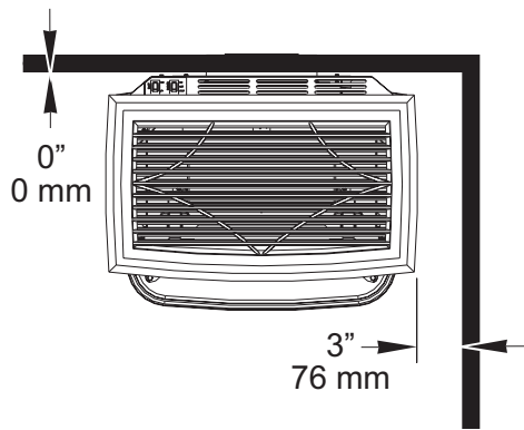
Figure 2. Parallel Installation Clearances.
