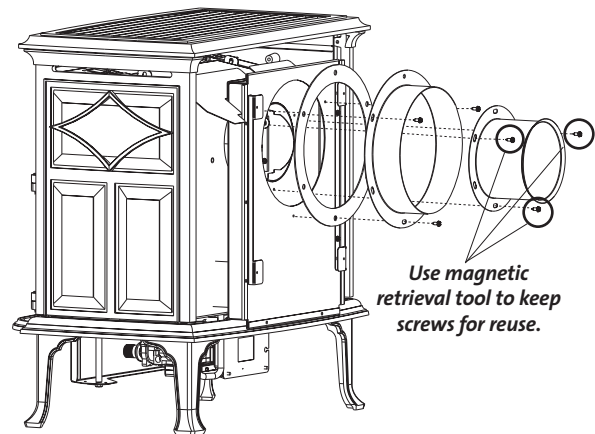
Figure 14. Remove the 5/8 Adaptor Collar components and replace with the 4/6 collar parts.
