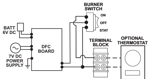
Figure 37. Accessory wiring diagram.
