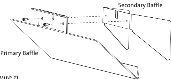
Figure 11. Remove the Primary Baffle from Secondary Baffle.
