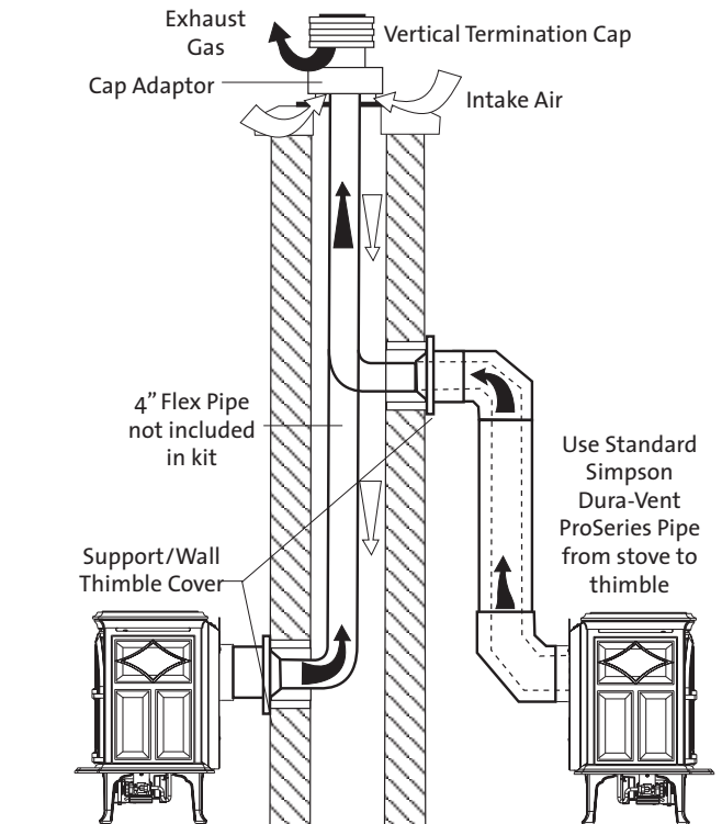
Figure 18. Vent System through a masonry chimney using the Simpson Dura-Vent Chimney Conversion Kits. Drawing is for illustrative purposes only - DO NOT VENT TWO APPLIANCES INTO A SINGLE CHIMNEY.
