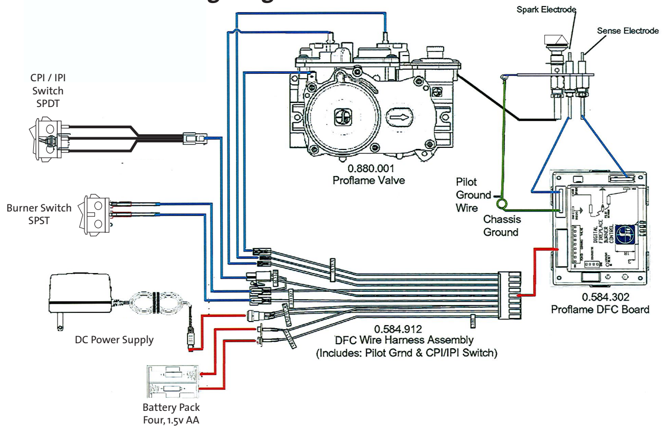
Figure 54. GF 200 DV IPI Proflame 1 Components
