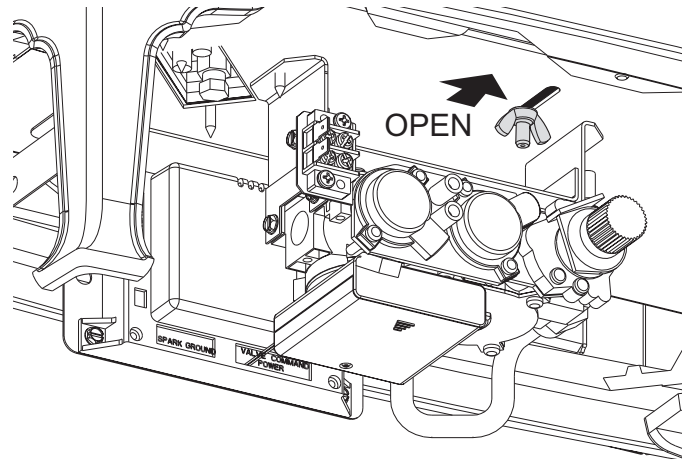
Figure 45. Loosen the wing nut to adjust the air shutter. Min. Opening NG: 1/16" (1.5 mm) Factory Setting Min. Opening LP: 1/8" (3 mm)
