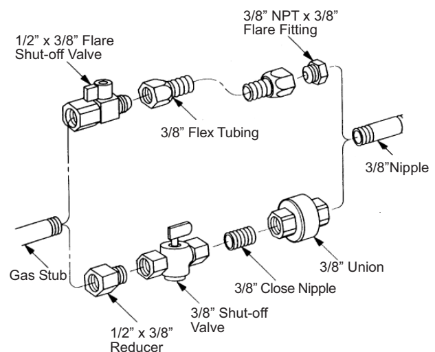
Figure 33. Supply valve connection fittings.
