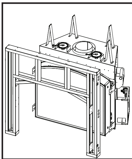
Figure 20: TC 36D arched frame assembled.
