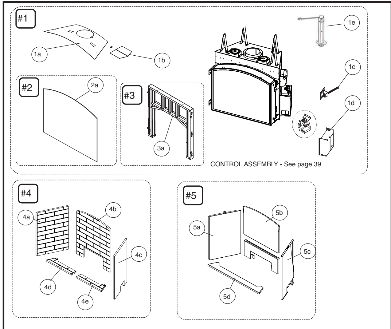
Figure 64: TC36 D Arched parts.
