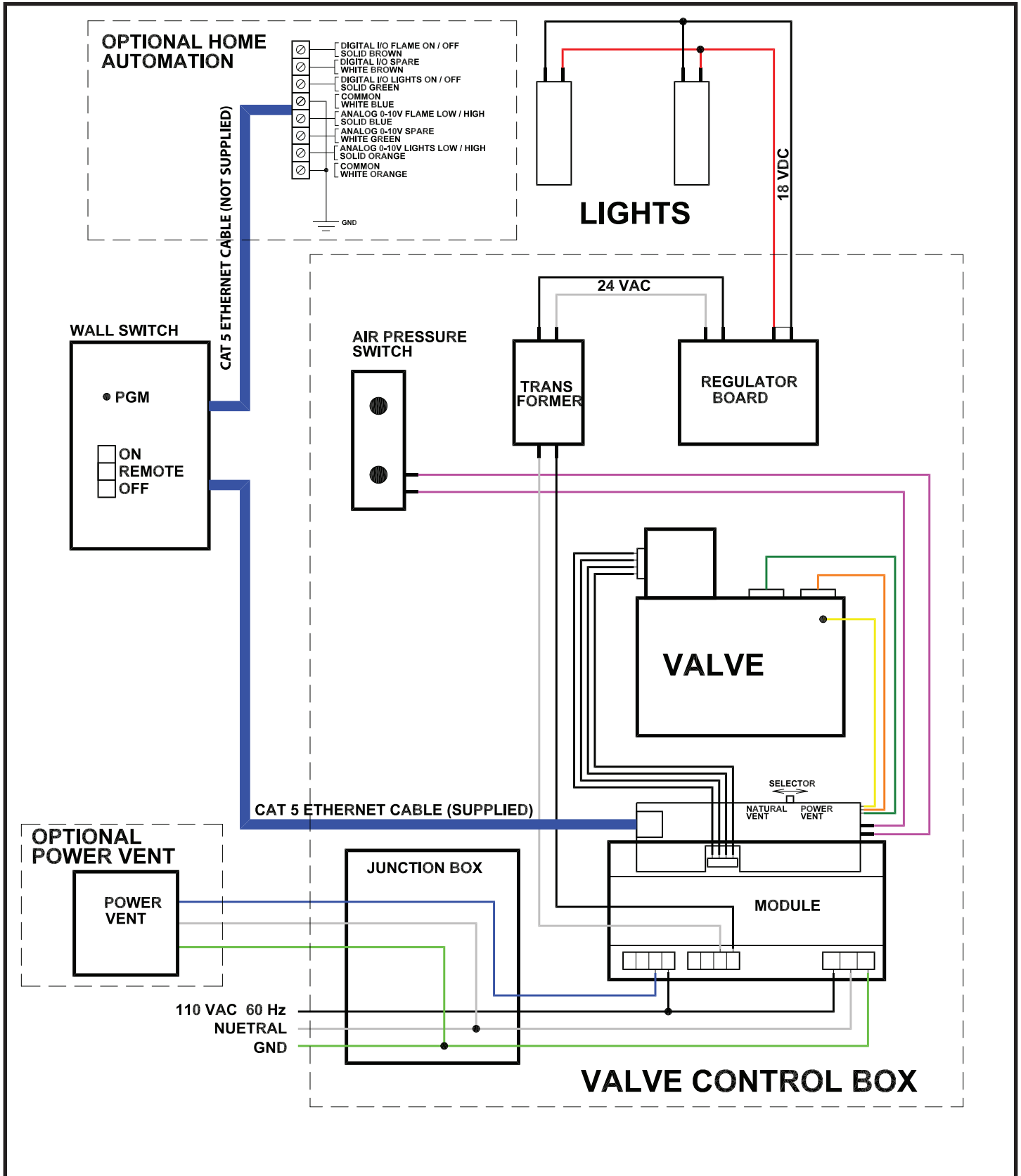
Figure 66: TC 36D Wiring diagram.
