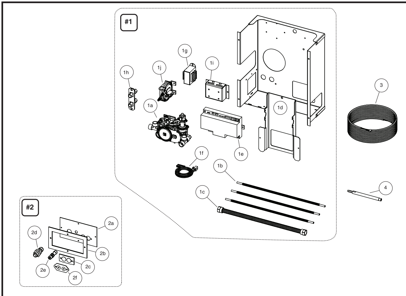
Figure 65: TC D Control assembly.
