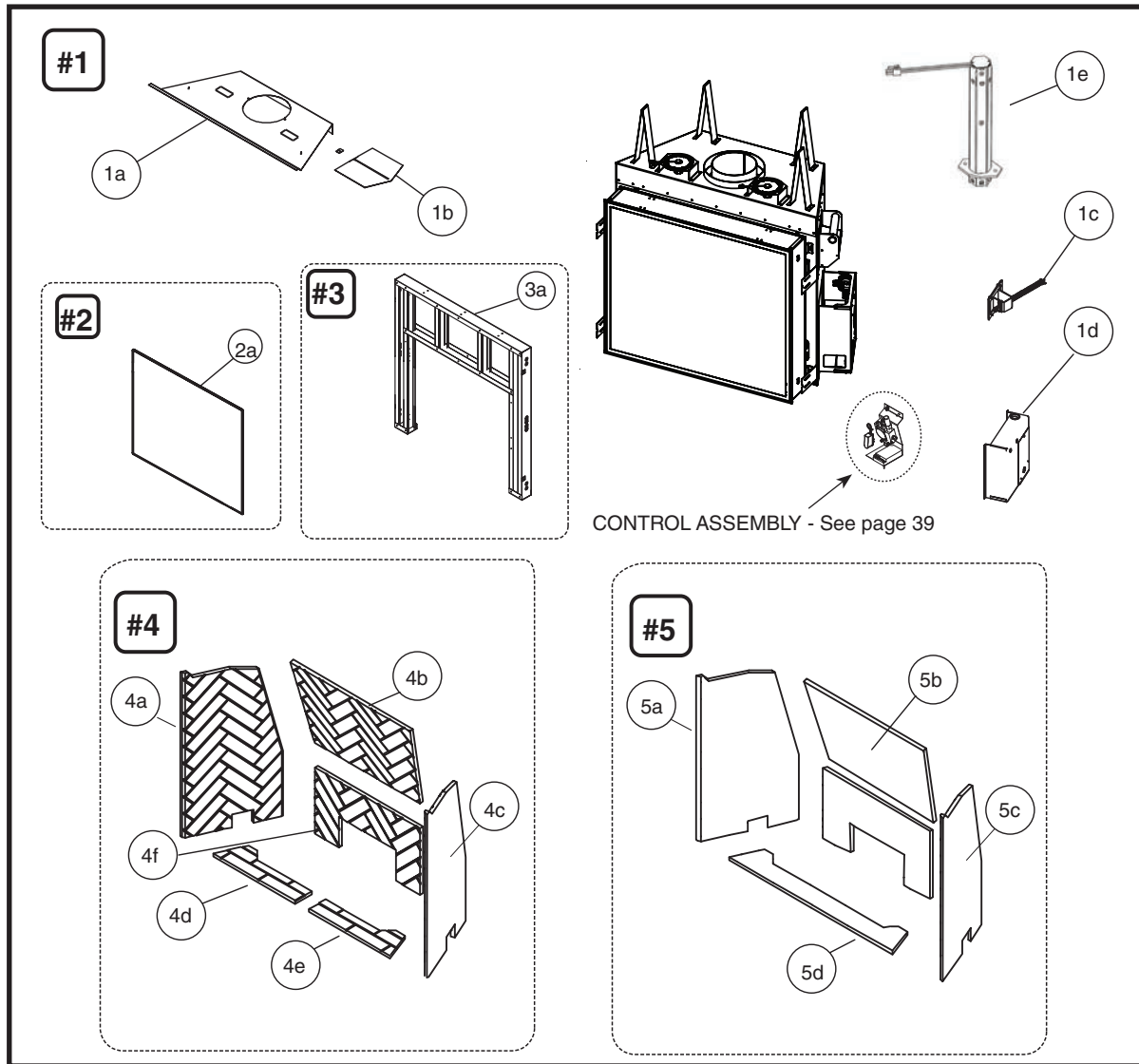
Figure 63: TC36 D parts.
