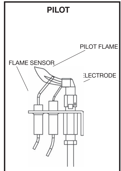
Figure 62: Pilot assembly.
