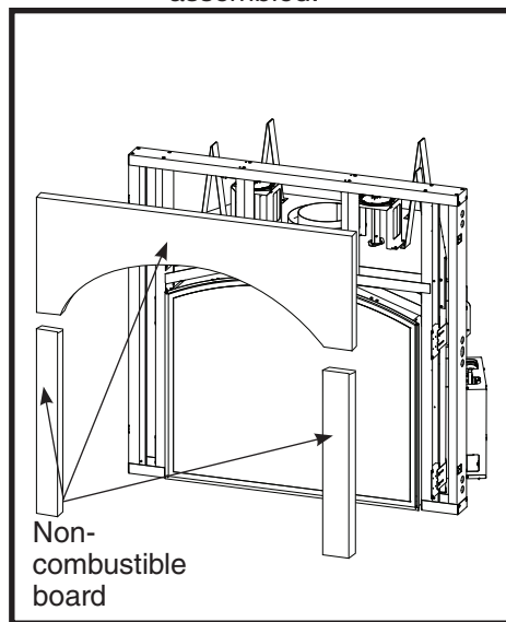
Figure 22: TC 36D arched frame with non-combustible board.
